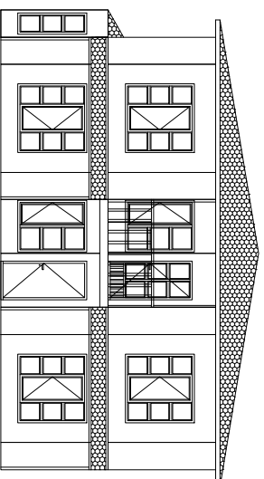
81 + 66 = 147 m 2 PREFABRIKE BINA PLANI
