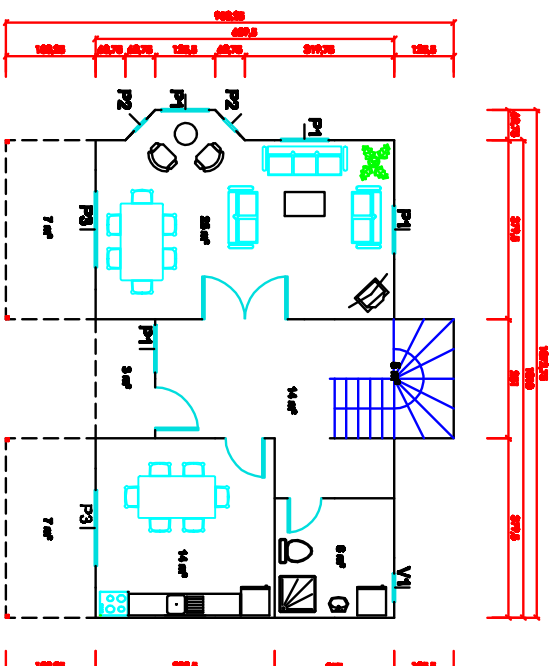
81 m 2 PREFABRIKE BINA ZEMİN KAT PLANI
