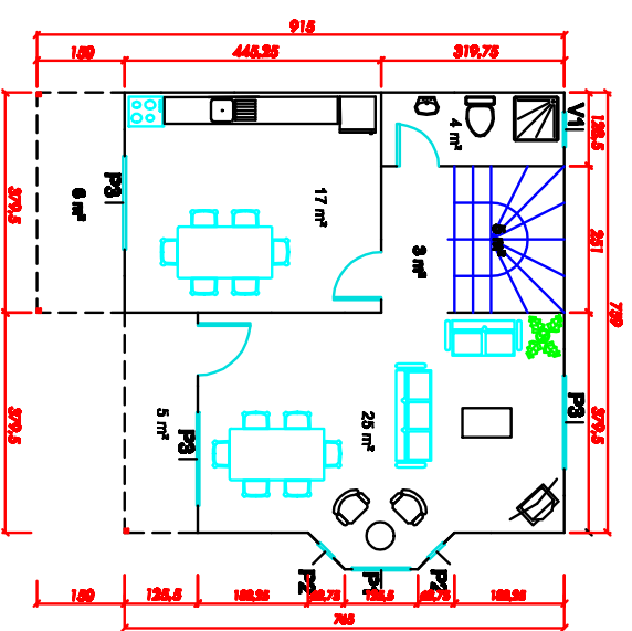
65 m 2 PREFABRIKE BINA ZEMİN KAT PLANI
