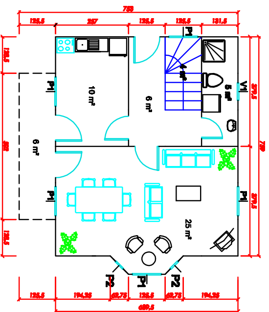
56 m 2 PREFABRIKE BINA ZEMİN KAT PLANI
